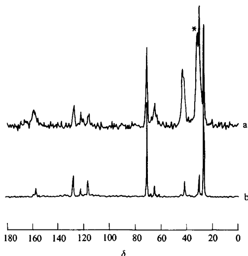
Fig.2 ^{13}\text{C} -NMR spectra of HDI-HB6-685 at 130 °C
